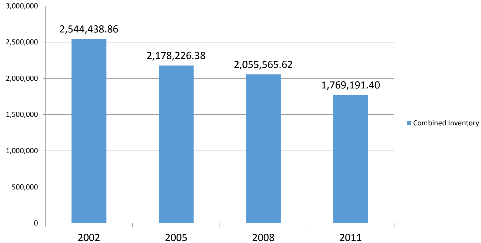
Statewide Emissions
