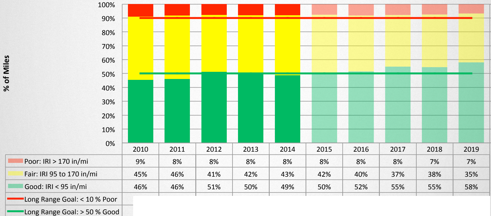
High Volume Pavement Condition (3,080 Mi/ 11,845 SA) Forecast with 148 Million / Yr
