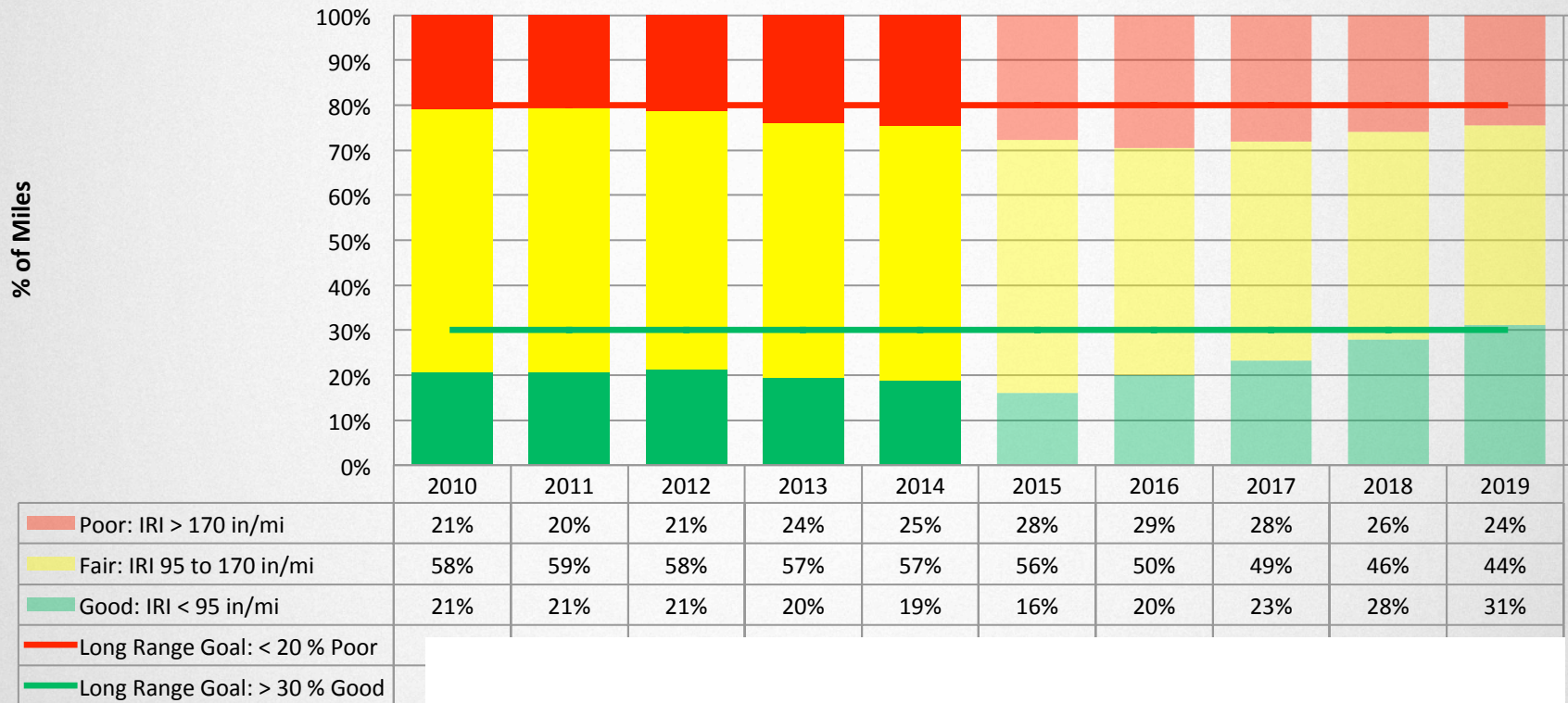
Low Volume Pavement Condition (1,865 Mi/ 4,410 SA) Forecast with 10 + 40 Million / Yr
