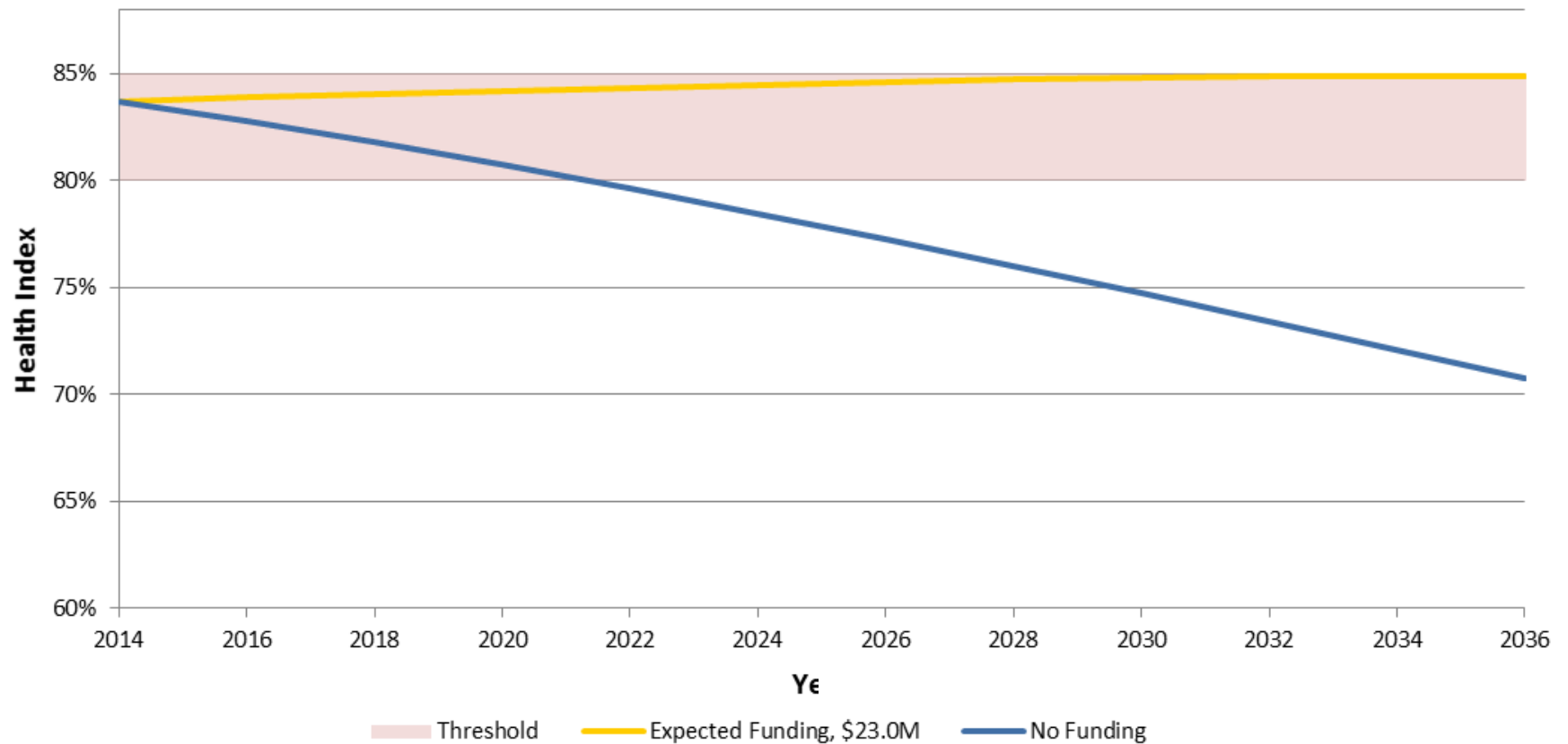
Projected System Health State Inventory
