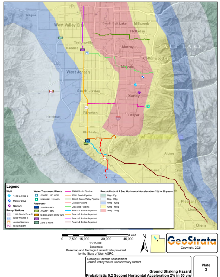
The Jordan Aqueduct has multiple segments that pass through ground acceleration zones. A large earthquake could damage and separate the pipeline.
