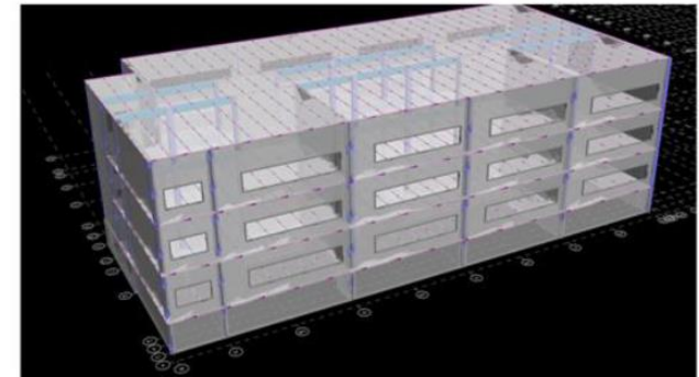
Figure 8 - RAM Model of the 1961 North Addition Building
