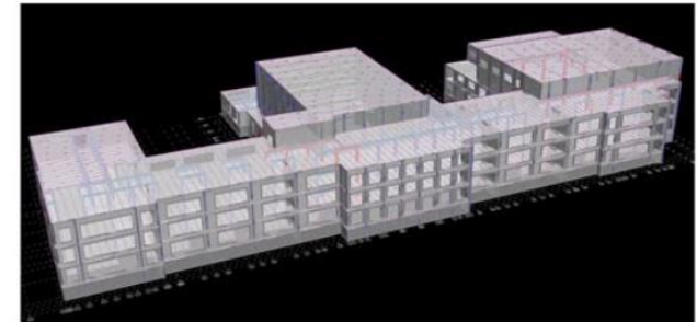
Figure 7 - RAM Model of the 1929 Original Building
